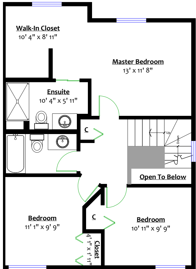
UPPER LEVEL Floor Area: 759 Sq. Ft.
