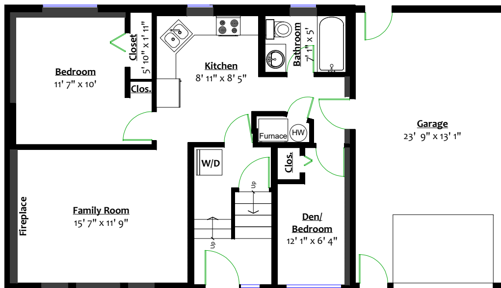
LOWER LEVEL Floor Area: 768 Sq. Ft.
