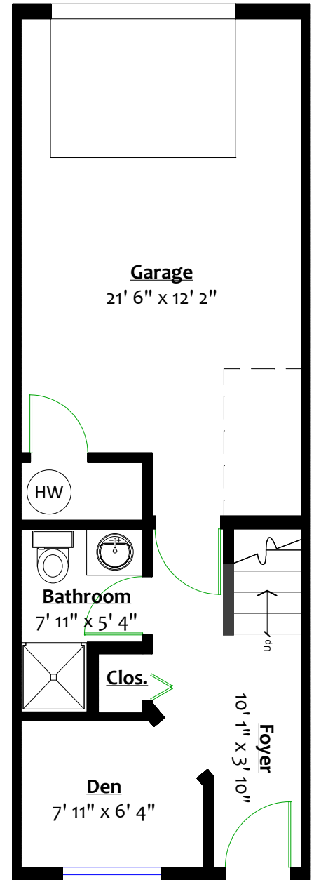
LOWER LEVEL Floor Area: 206 Sq. Ft. Ceiling Height: 8'
