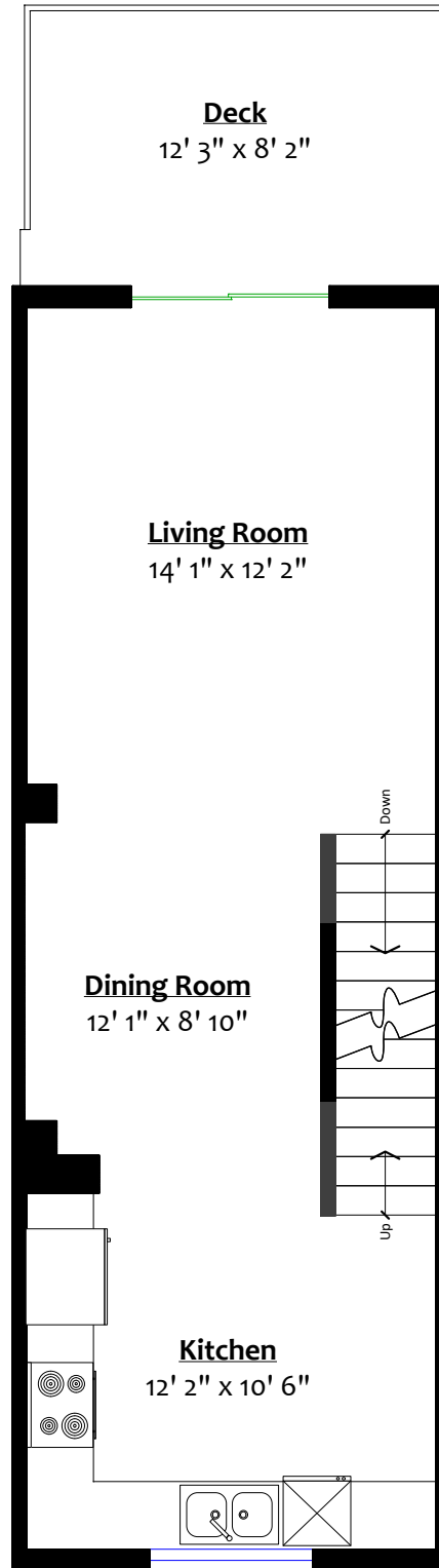
MAIN LEVEL Floor Area: 488 Sq. Ft. Ceiling Height: 9'
