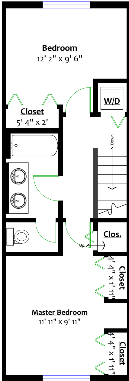
UPPER LEVEL Floor Area: 488 Sq. Ft. Ceiling Height: 8'
