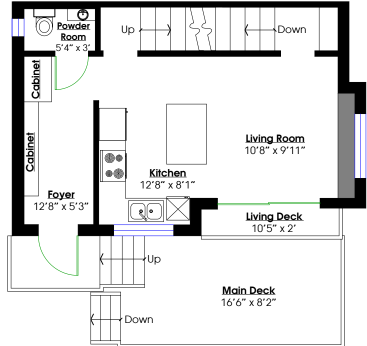
MAIN LEVEL Floor Area: 435 Sq. Ft. Ceiling Height: 9'11"
