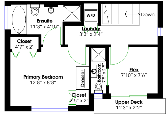
UPPER LEVEL Floor Area: 426 Sq. Ft. Ceiling Height: 8'
