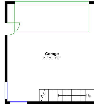
DETACHED GARAGE Floor Area: 449 Sq. Ft. Ceiling Height: 8'10"
