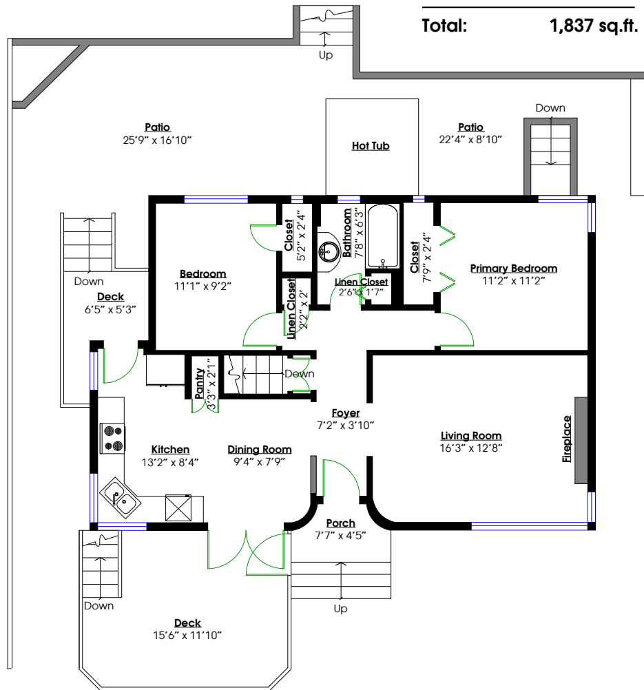
MAIN LEVEL Floor Area: 907 Sq. Ft. Ceiling Height: 8'3"
