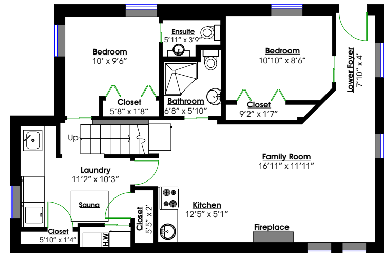
LOWER LEVEL (under-height) Floor Area: 913 Sq. Ft. Ceiling Height: 6'11"
